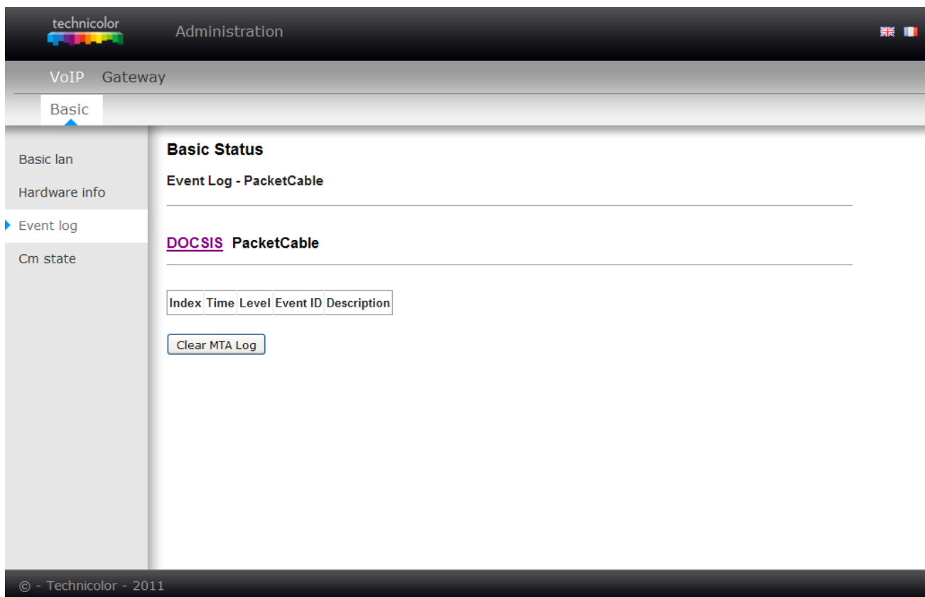
Fig. 2-48 VoIP\Basic\Event log\PacketCable
