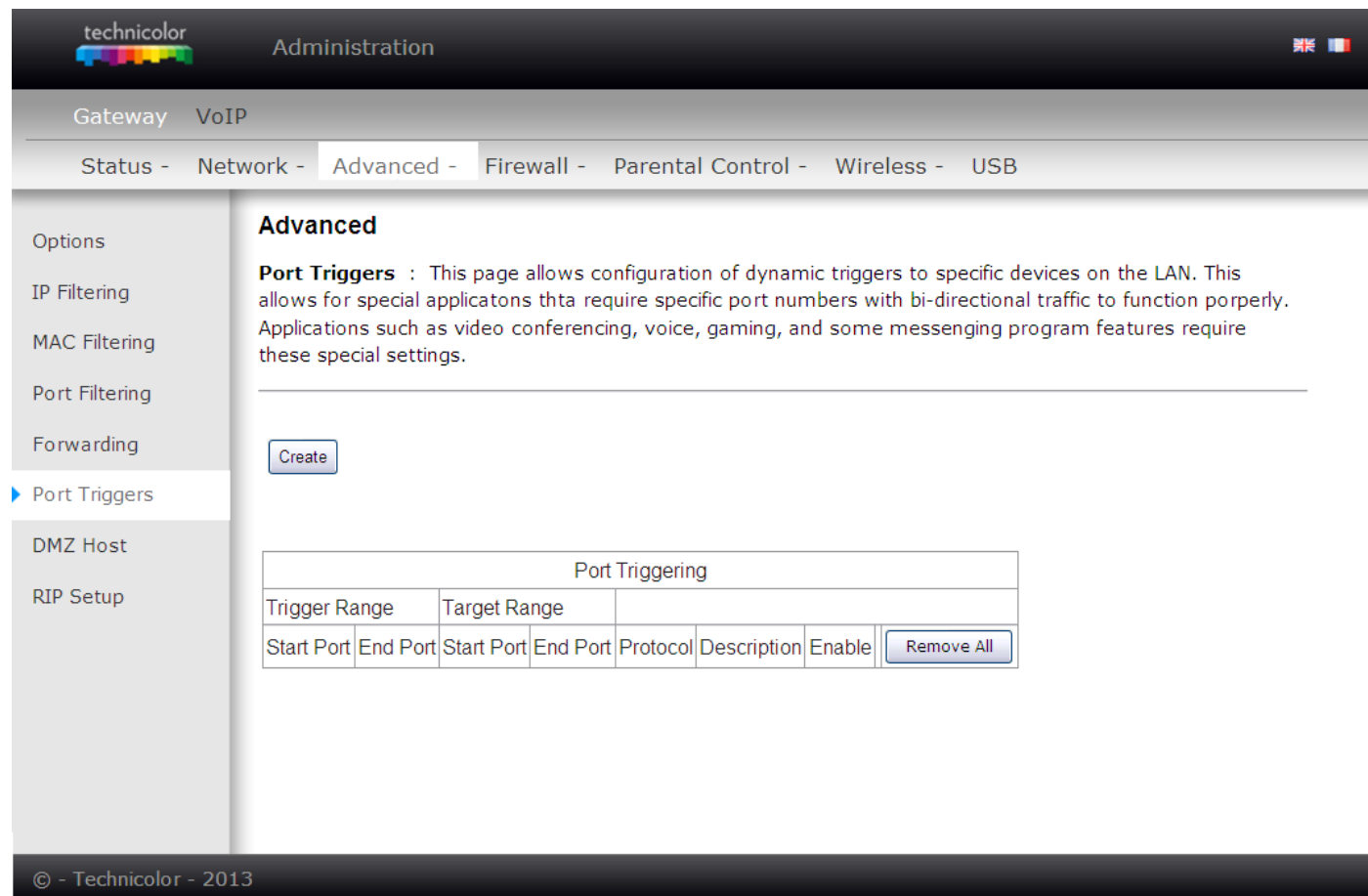
Fig.2-23 Gateway\Advanced\Port Triggers
